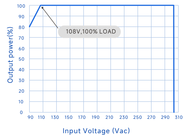
Output Power Vs. Input Voltage
